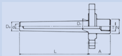
WL08 溶接形
