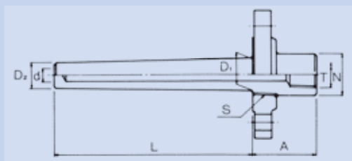
WL07 溶接形
